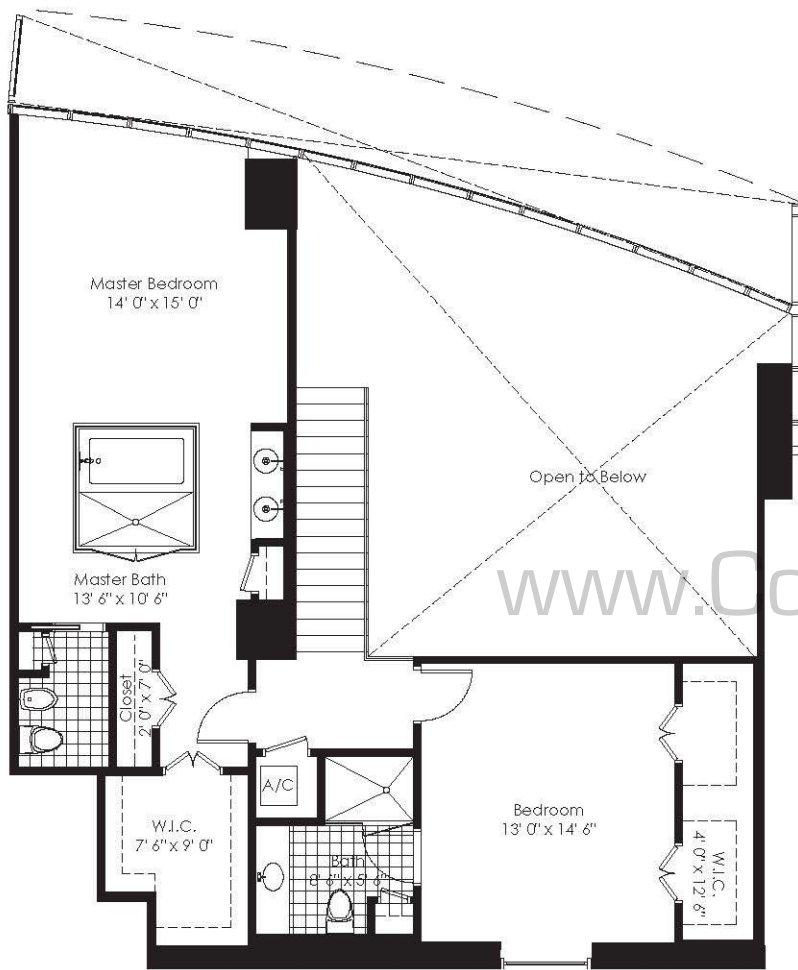
Upper Level
